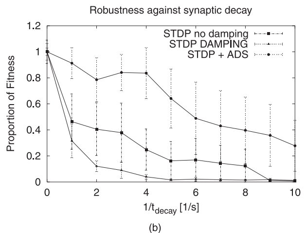
Figure 3 Fitness and robustness. (a) Average fitness of the best individual in the last generation; (b) robustness against synaptic decay; t_{\text{decay}} indicates the speed with which weights decay exponentially to 0.
