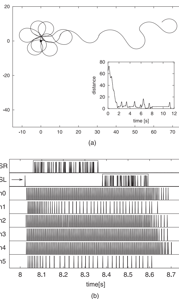
Figure 4 Evolved robot using STDP+ADS. (a) Trajectory, inset: distance to light source, (b) network activity during a fraction of the trajectory triggered by a single spike. SL: left sensor; SR: right sensor; n0–n5: neurons 0–5.
